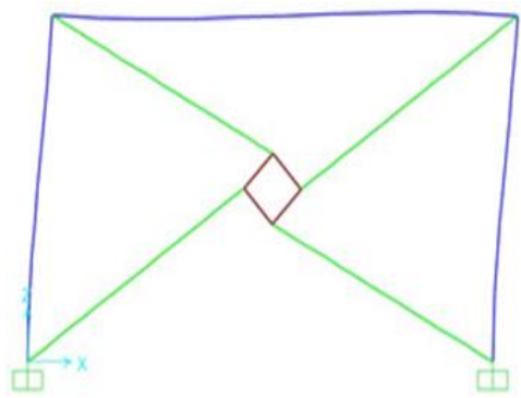
Fig. 1: Deformed configuration of the system
