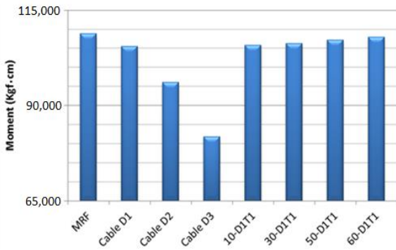
Fig. 14: Bending moments of the beams
