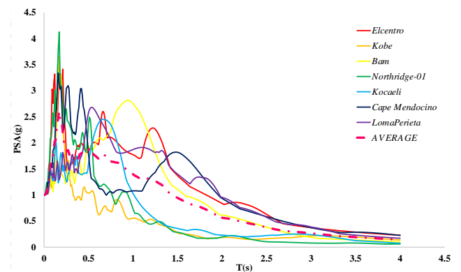
Fig. 8: Design Spectrum and the average of the scaled spectra
