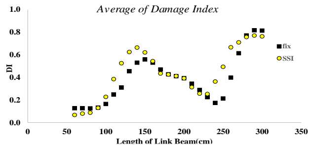
Fig. 12: Average of DI Values (According to frame’s primary design)
