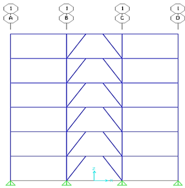
Fig. 1: elevated view of the frame in SAP2000
