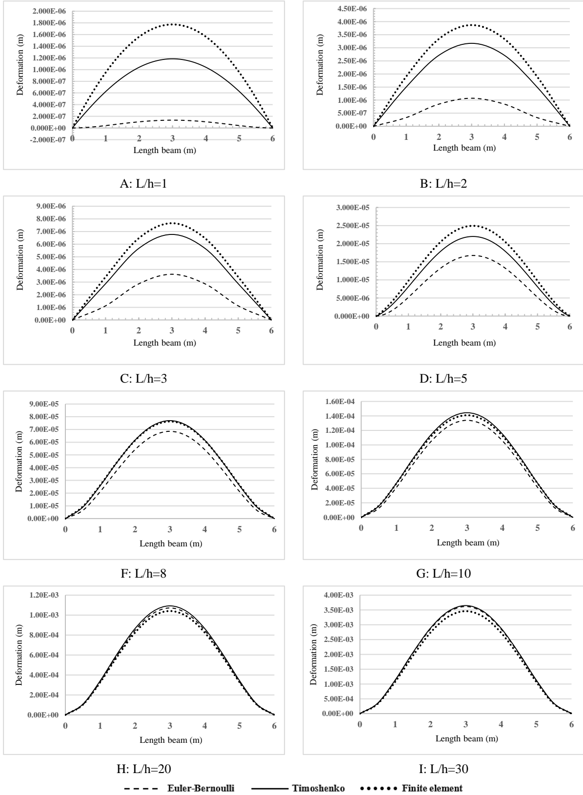
Fig. 5: The deflection of the fixed-fixed beam under uniform distributed load
