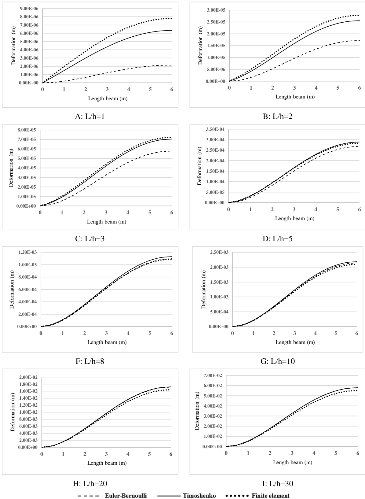
Fig. 8: The deflection of the fixed- sliding beam under uniform distributed load
