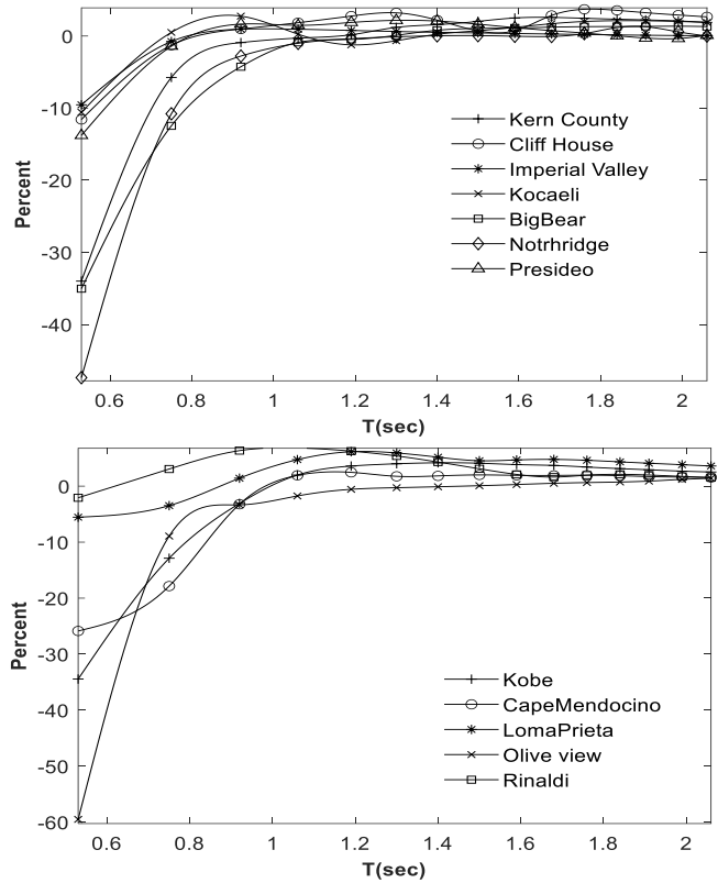
Fig. 13: The RMS acceleration reduction by the fuzzy compared to
