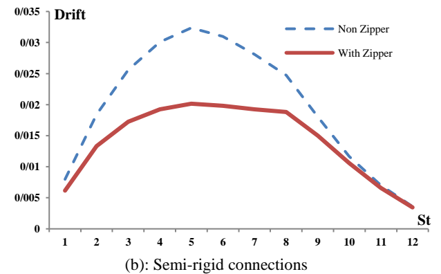
Fig. 7: Diagram of reduction in the relative story displacement in a 12- story frame with a zipper bracing system relative to a Chevron bracing system under Takarazuka record.
