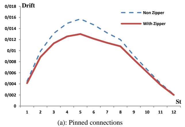
Fig. 6: Diagram of reduction in the relative story displacement in a 12- story frame with a zipper bracing system relative to a Chevron bracing system under Parkfield record.
