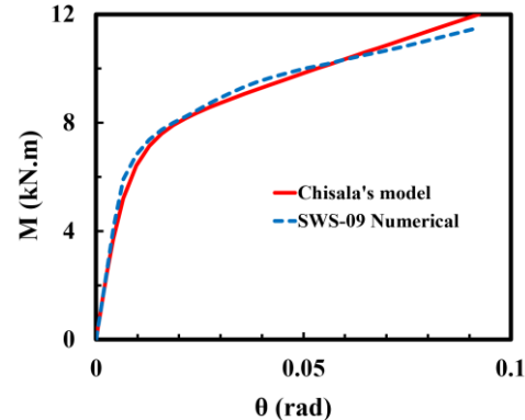
Fig. 72: Numerical and analytical moment-rotation curves for SWS-09 specimen.
