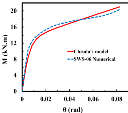
Fig. 69: Numerical and analytical moment-rotation curves for SWS-06 specimen.
