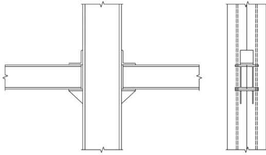
Fig. 11: Cross-shaped setup for stiffened welded-seat (SWS) connections.
