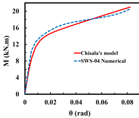
Fig. 67: Numerical and analytical moment-rotation curves for SWS-04 specimen.
