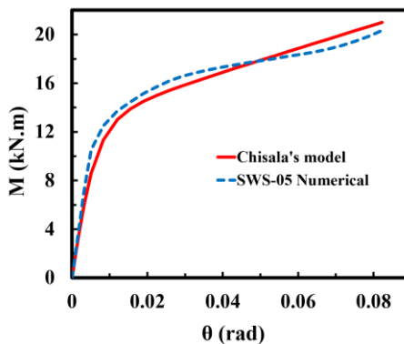
Fig. 68: Numerical and analytical moment-rotation curves for SWS-05 specimen.
