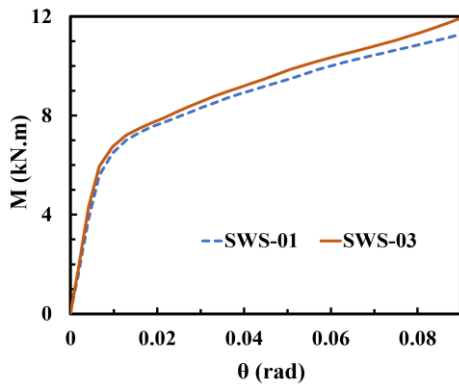
Fig. 84: Effects of the triangular stiffener thickness on the moment-rotation curve.
