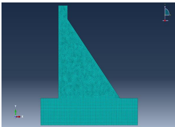
Fig. 15: The meshing of the concrete dam structure
