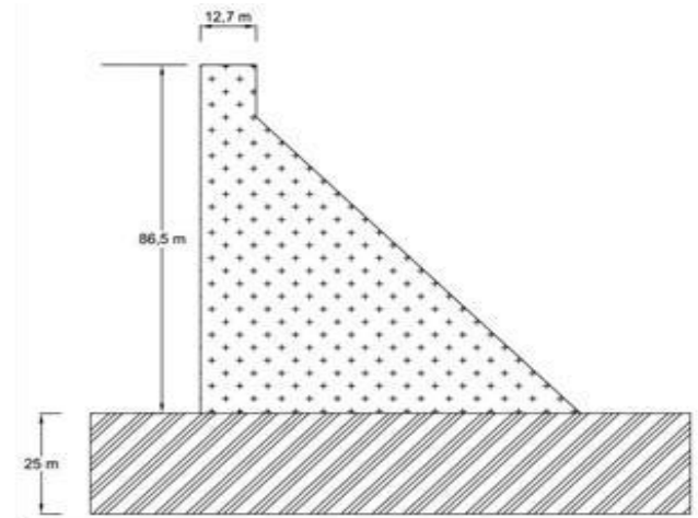
Fig. 7: Cross-section of Zhavveh rolled concrete dam [13]
