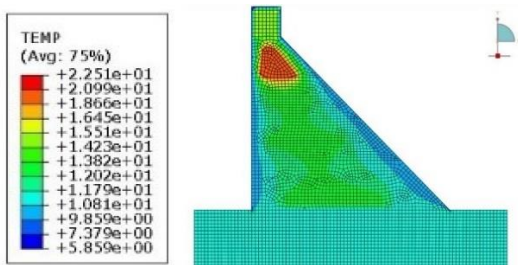
Fig. 19: The maximum temperature generated at the level of 86.5 meters (173 layers) - Project started in October
