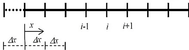
Fig. 3: One-dimensional mesh for finite difference approximation.
