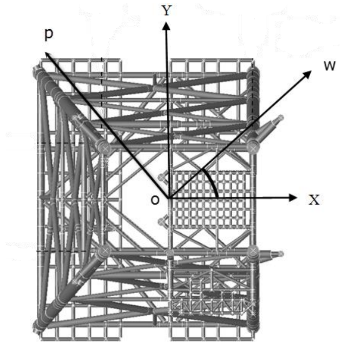
Fig. 4: Structural axes and rotational system
