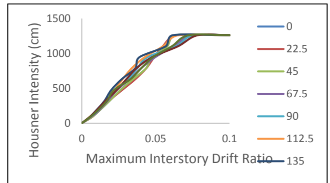
Fig. 5: MIDA diagrams for one record in all directions
