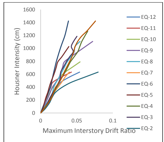
Fig. 6: diagrams of MIDA results (the earthquake is applied along the principal axes) for all EQs
