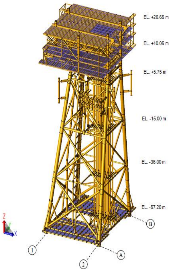
Fig. 1: SPD13 wellhead platform sags model
