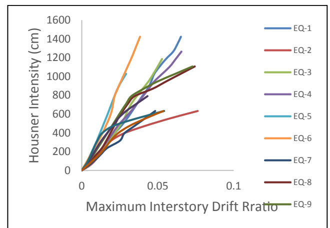
Fig. 7: diagrams of DMIDA results for maximum EDP
