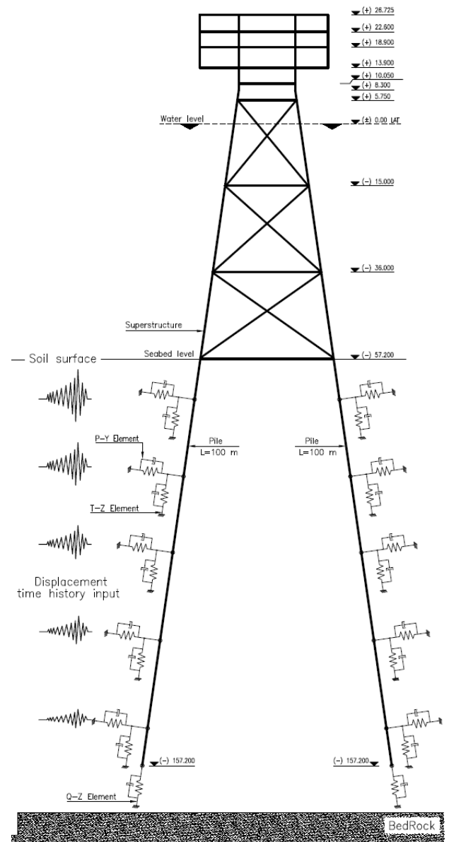
Fig. 2: Schematic view of SPD13 wellhead platform
