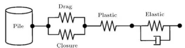
Fig. 3: Components of nonlinear p-y elements
