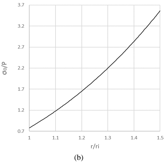
Fig. 7: The variation of normalized stresses versus normalized radial distance for the second model, (a) Radial stress, (b) Hoop stress.
