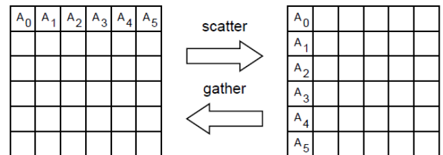
Fig. 2: The illustration of MPI_GATHER and MPI_SCATTER functions [26]
