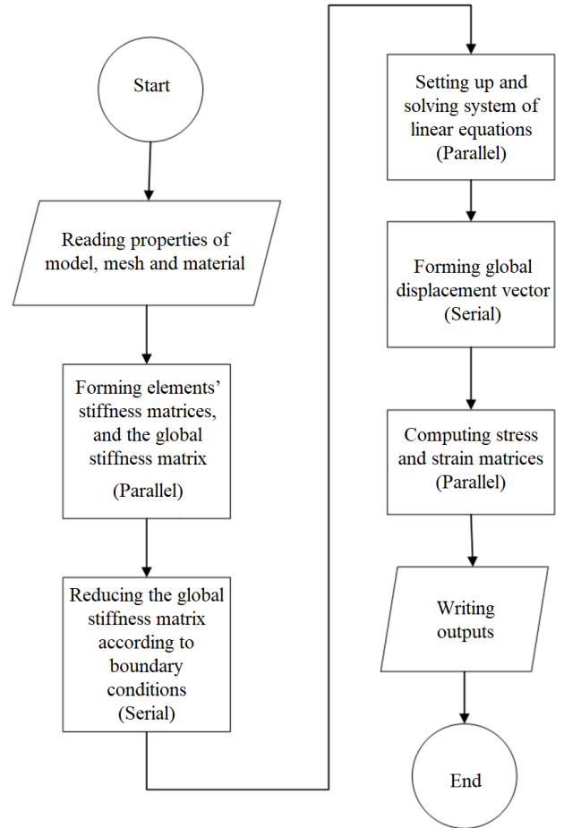
Fig. 5: The flowchart of Finite Element Analysis
