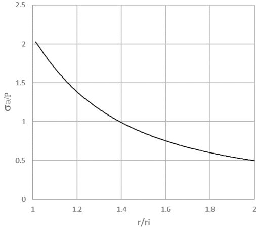
Fig. 6: The variation of normalized stresses versus normalized radial distance for the first model, (a) Radial stress, (b) Hoop stress.
