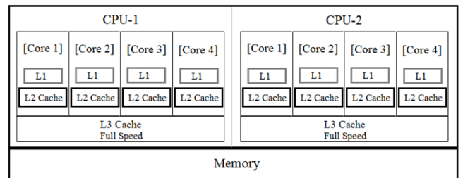
Fig. 9: An overview of CPUs and levels of CPU caches
