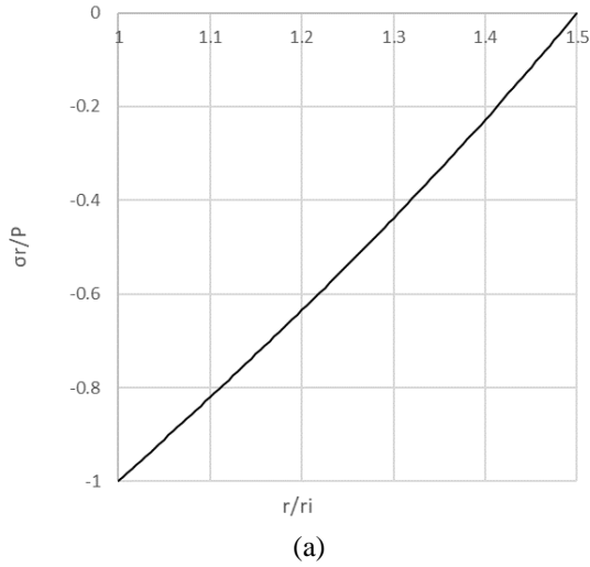
Fig. 6: The variation of normalized stresses versus normalized radial distance for the first model, (a) Radial stress, (b) Hoop stress.
