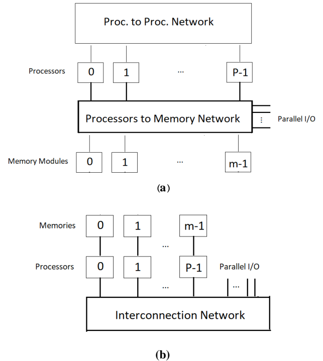
Fig. 1: A parallel processor with (a) shared memory, (b) distributed memory
