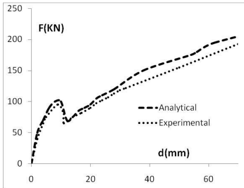
Fig.6: Load-displacement curve (Specimen N2)
