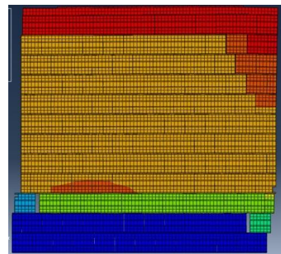
Fig.12: Failure mode of N2-C2
