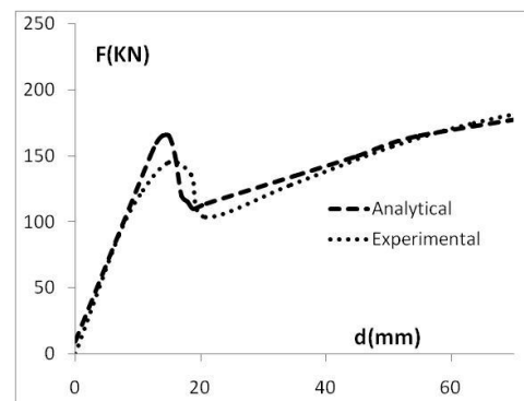
Fig.4: Load-displacement curve (Specimen I)
