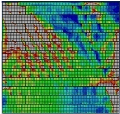
Fig.15: Combined stress of N2-C2
