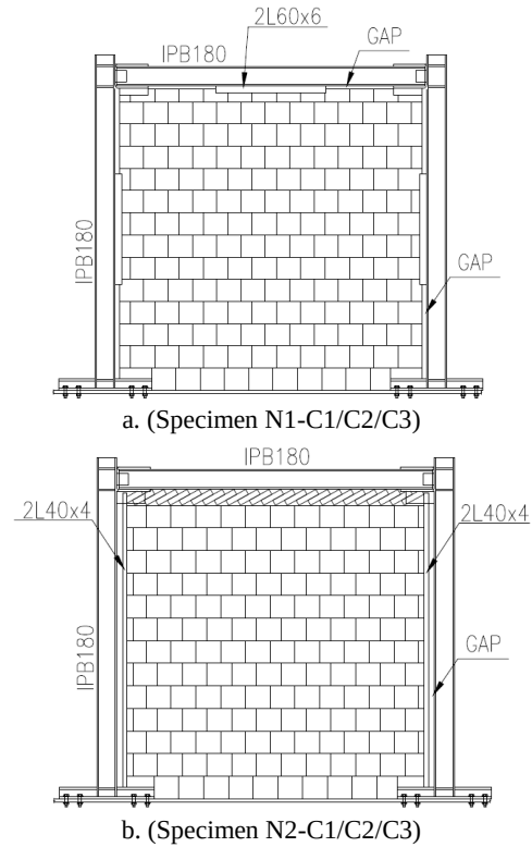
Fig.10: The details of numerical specimens
