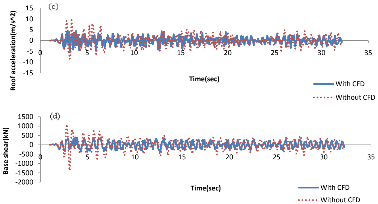
Fig.9: Response of the frame with and without damper: a) displacement of the roof, b) velocity of the roof, c) acceleration of the roof, d) Base shear.
