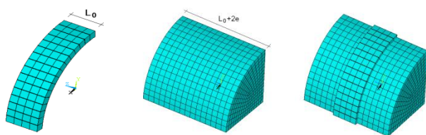
Fig. 2: Finite element model of CFD a)Cylinder; b) Solid shaft; c)Assembled CFD
