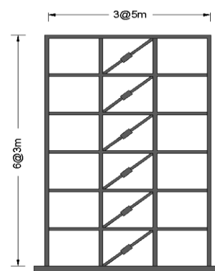
Fig.5: Elevation of the 6-storey frame
