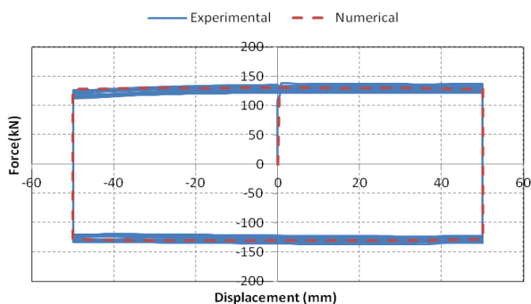
Fig. 4: The experimental hysteretic behavior of a CFD specimen with design slippage load of 130kN.
