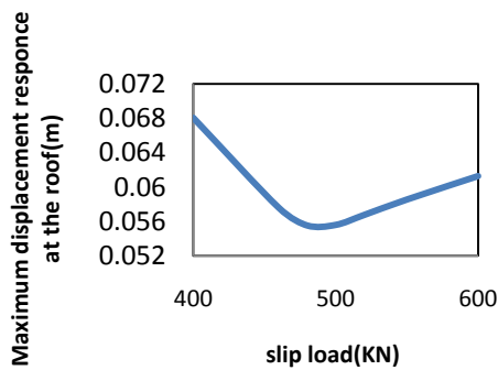
Fig. 6: Maximum displacement at the top of the frame versus slippage load
