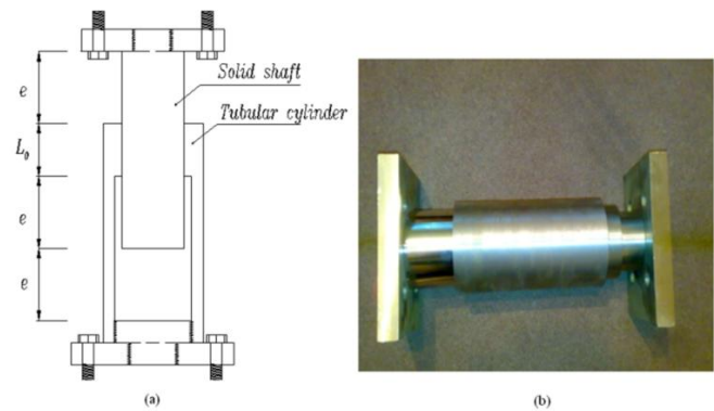
Fig. 1: a) Longitudinal section of CFD; b) Manufactured CFD [8]
