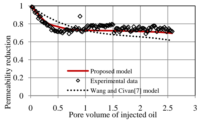
Fig.8: Experimental and simulated permeability reduction during primary deposition ( Q=1 cc/hr) in sandstone core sample [24, 25]
