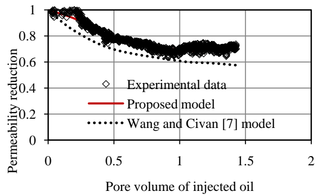
Fig.9: Experimental and simulated permeability reduction during primary deposition ( Q=1 cc/hr) in carbonate core sample [24, 25]
