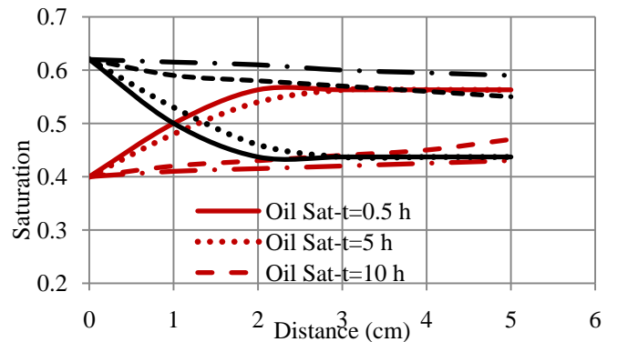
Fig.14: Saturation profiles at different time steps in carbonate core sample ( Q=1 cc/hr) [24, 25]
