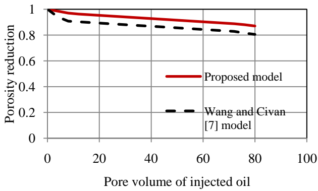
Fig.7: Porosity reduction versus pore volume oil injected for oil GF3[11]
