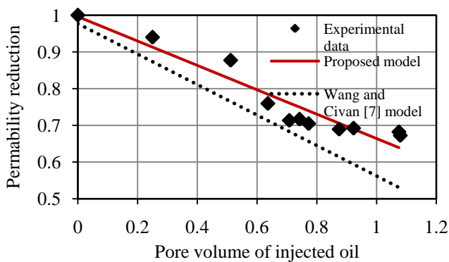
Fig.12: Experimental and simulated permeability reduction during primary deposition ( Q=10 cc/hr) in carbonate core sample [24, 25]
