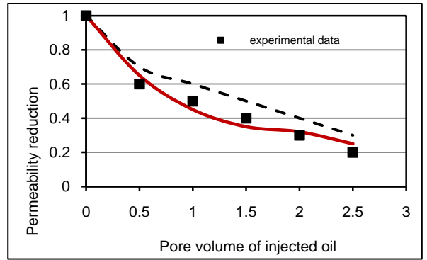
Fig.13: Comparison of the performance of the proposed model and model based on two phases black oil [24, 25]
