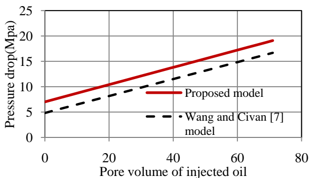
Fig.3: Pressure drop versus pore volume oil injected for oil GF3 [11]
