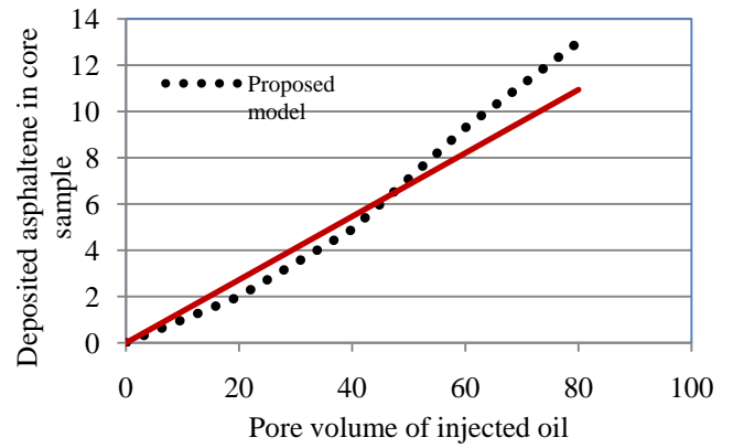
Fig.4: Deposited asphaltene in core sample versus pore volume of injected oil[11]
