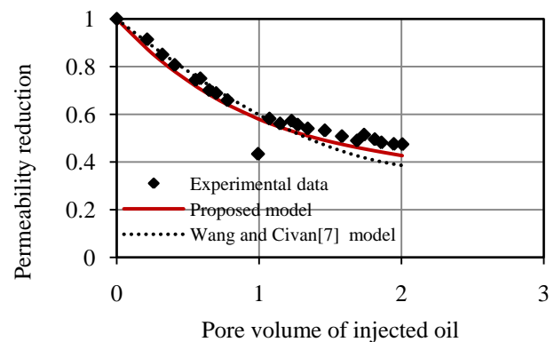
Fig.10: Experimental and simulated permeability reduction during primary deposition ( Q=3 cc/hr) in dolomite core sample [24, 25]
