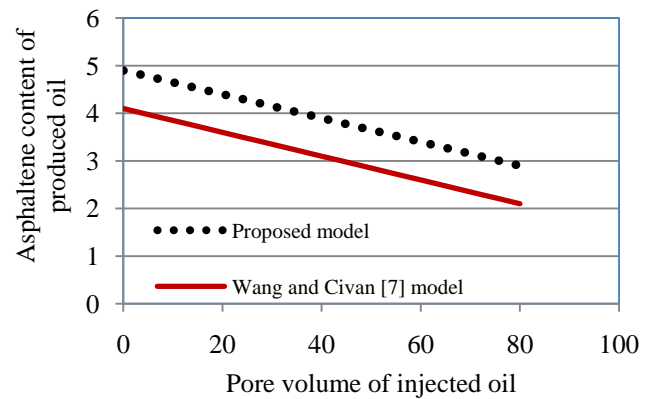
Fig.5: Asphaltene content of produced oil versus pore volume of injected oil[11]
