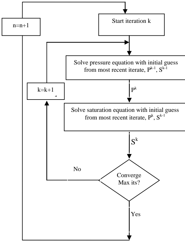
Fig.2: The iterative coupling approach for solving pressures and saturations
