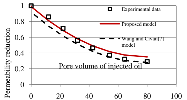
Fig.6: Permeability reduction versus pore volume oil injected for oil GF3[11]
