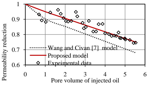
Fig.11: Experimental and simulated permeability reduction during primary deposition ( Q=10 cc/hr) in sandstone core sample [24, 25]
