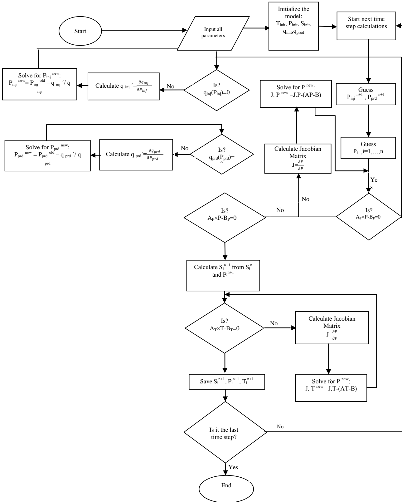
Fig.1: The IMPES method Flow Chart
