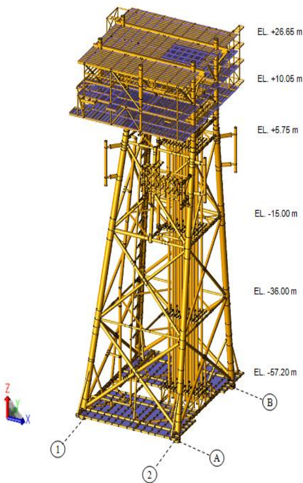
Fig. 1: SPD13 wellhead platform sacs model
