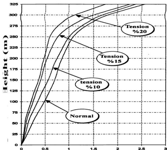
Fig.5-a: Max. displacement along tower(m)
