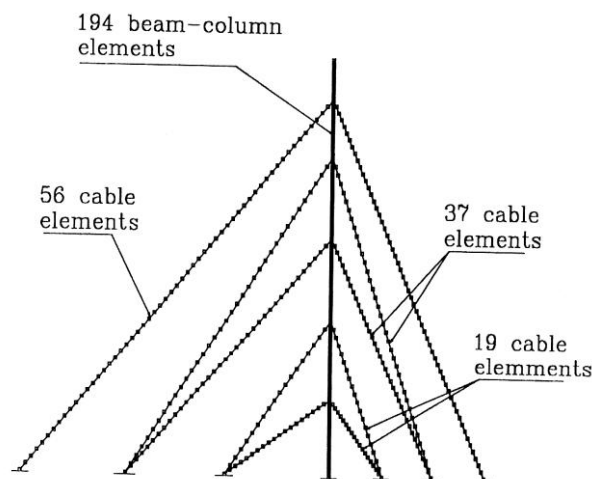
Fig. 4-b: Cables & beam-column Equivalent elements
