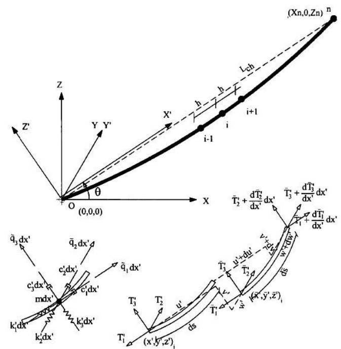
Fig.1: Cable element
