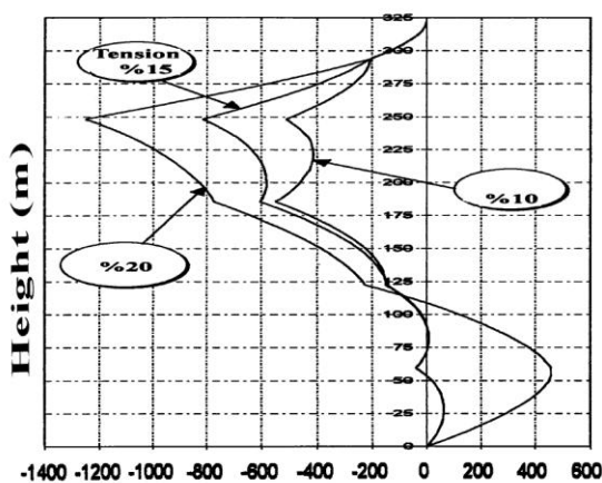
Fig.5-b: Moment along tower(ton-m)
