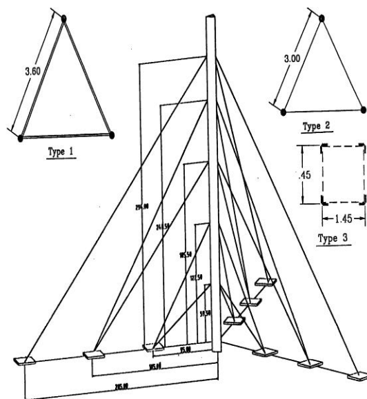
Fig. 4-a: Tower and space truss cross sections
