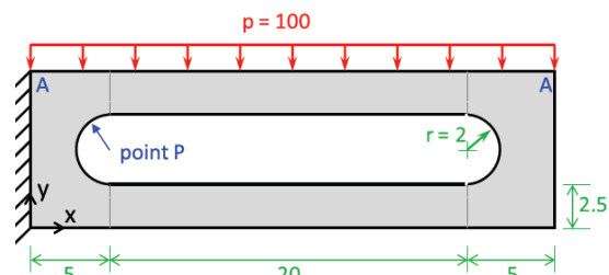
Fig. 7: Conditions of a 2D tool jig problem
