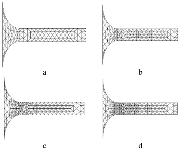
Fig. 4: Meshing during problem solving via proposed method
