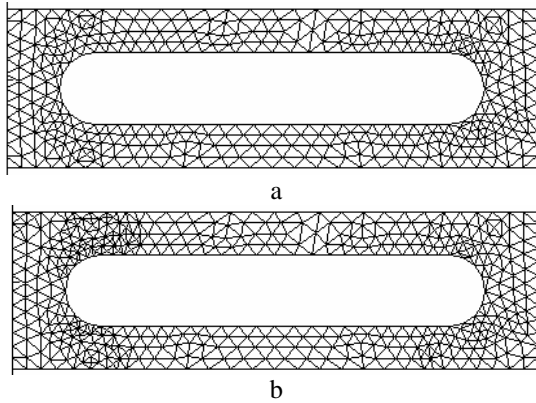
Fig. 8: Meshing during problem solving via proposed method
