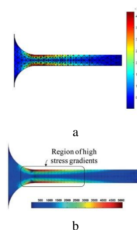
Fig. 6: Comparison of the results based on von Mises stress distribution
