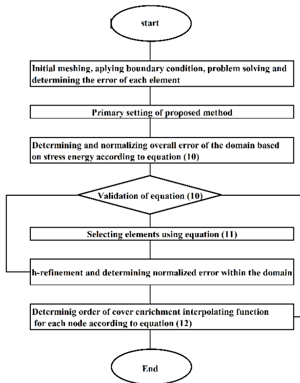
Fig. 2: Flowchart of hp-refinement method.
