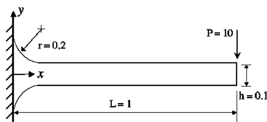
Fig. 3: Conditions of a cantilever beam having curved boundaries
