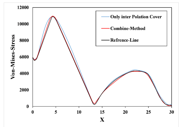
Fig.10: Comparison of the results based on von Mises stress distribution
