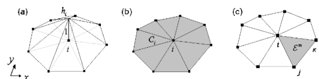
Fig. 1: A description of relationships among enriched subdomains using cover interpolation functions: a) linear interpolation function; b) covered region or elements affected by the by cover interpolation functions; and c) an enriched element.
