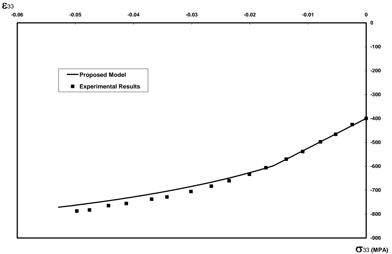
Fig.11: Comparison of the proposed model with results of 200 MPa confinement experiment
