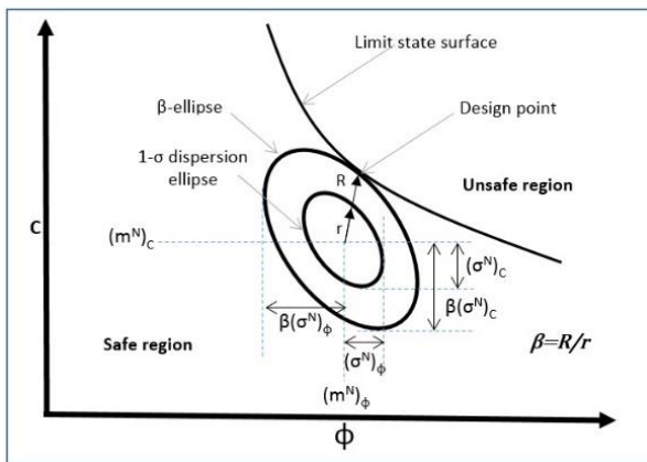
Fig. 1: In-plane equivalent normal ellipsoids and design point [17]
